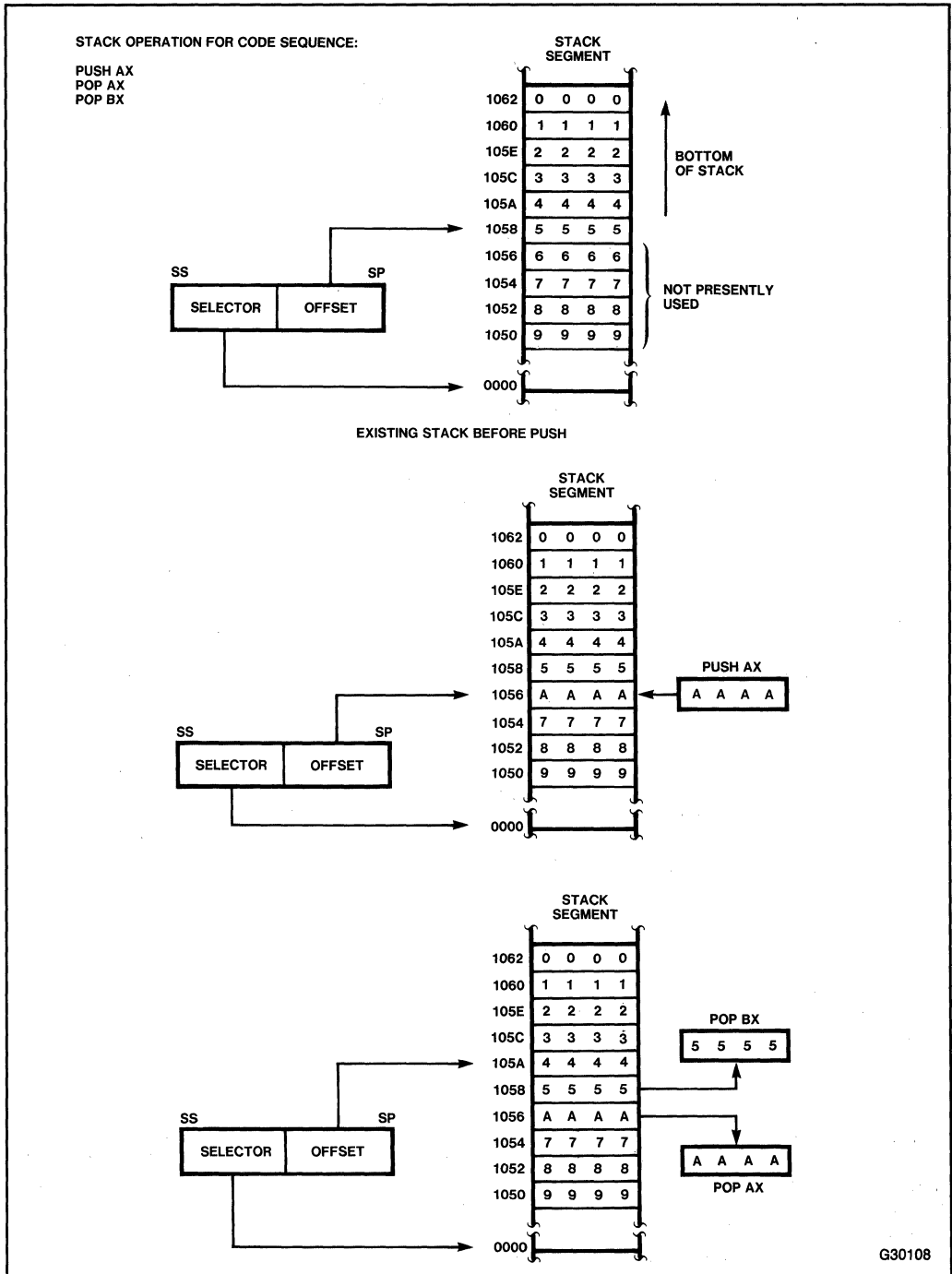
Figure 2-8. Stack Operation
