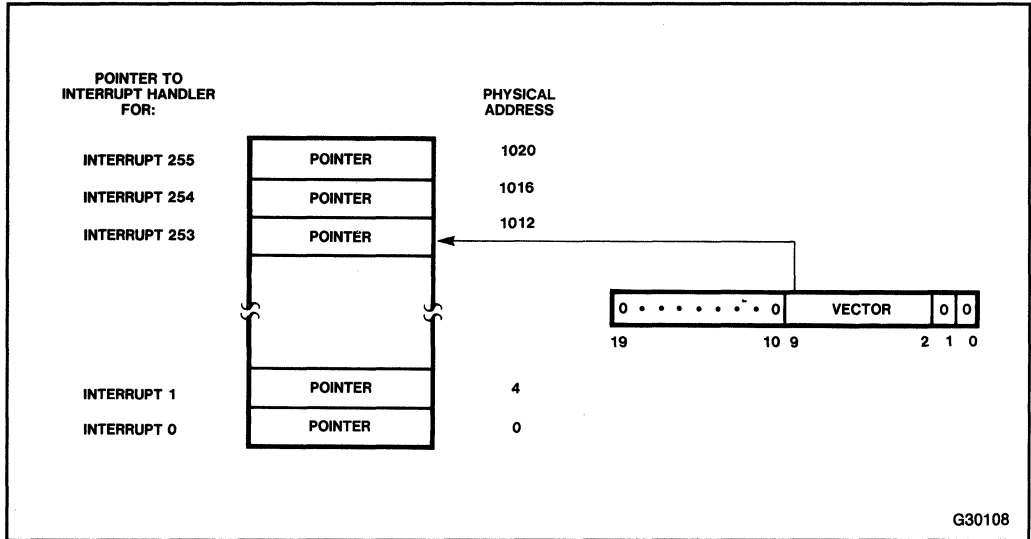
Figure 5-3. Interrupt Vector Table for Real Address Mode
