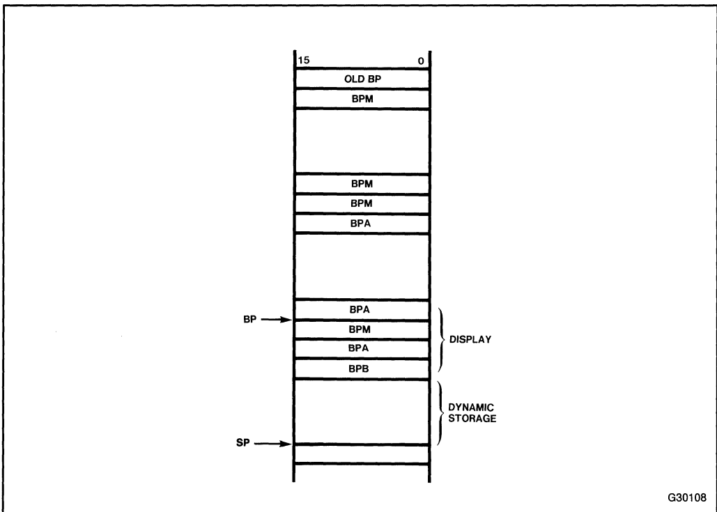
Figure 4-2c. Stack Frame for Procedure B at Level 3 Called from A
