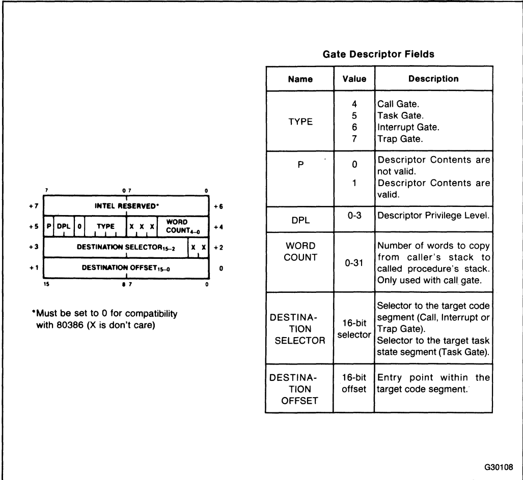
Figure 7-10. Gate Descriptor Format
