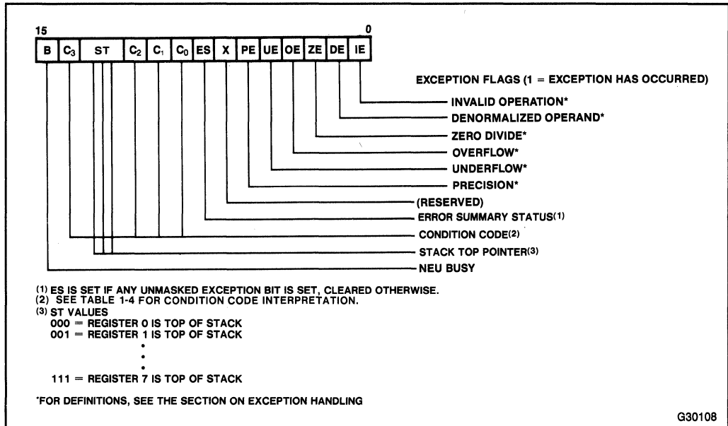
Figure 1-4. 80287 Status Word
