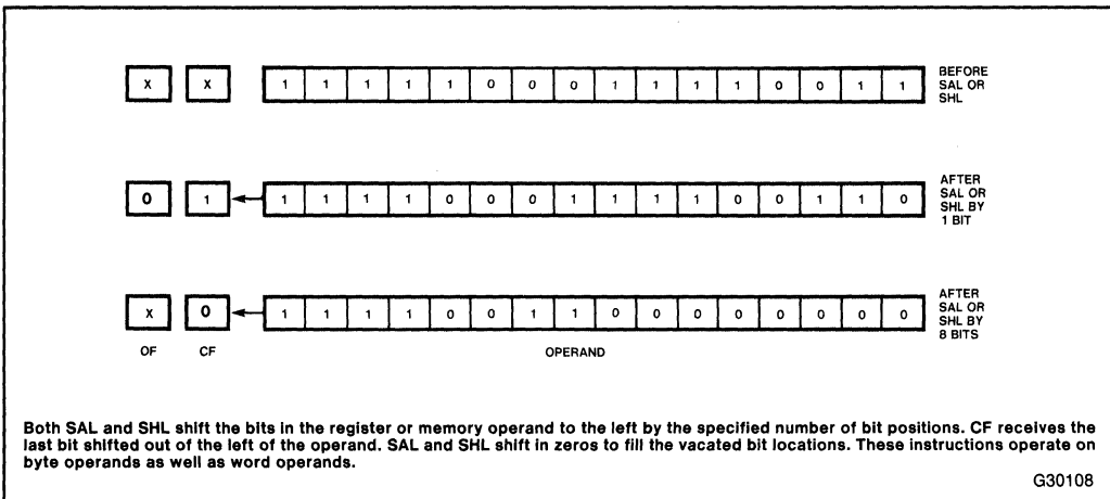
Figure 3-6. SAL and SHL
