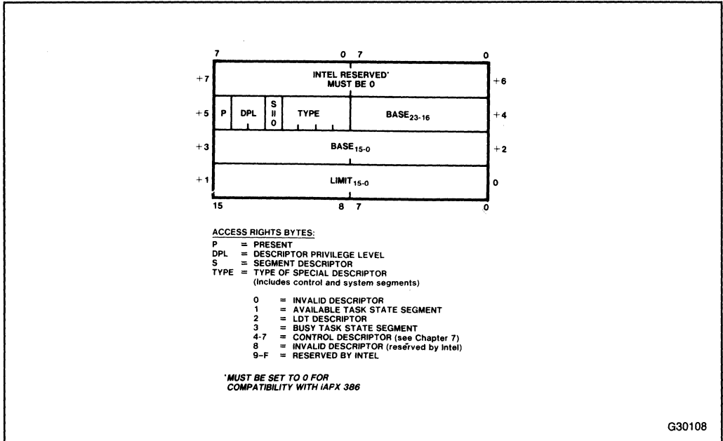
Figure 6-4. System Segment Descriptor or Gate Descriptor (S = 0)
