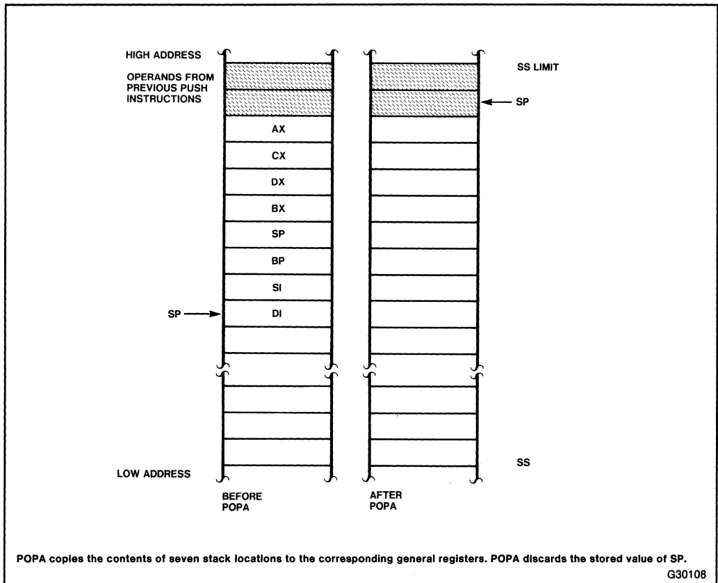
Figure 3-4. POPA
