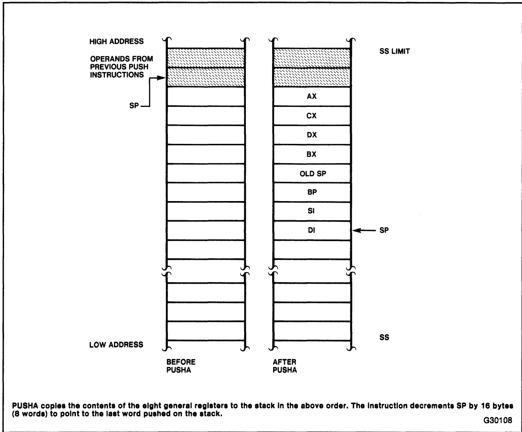
Figure 3-2. PUSHA
