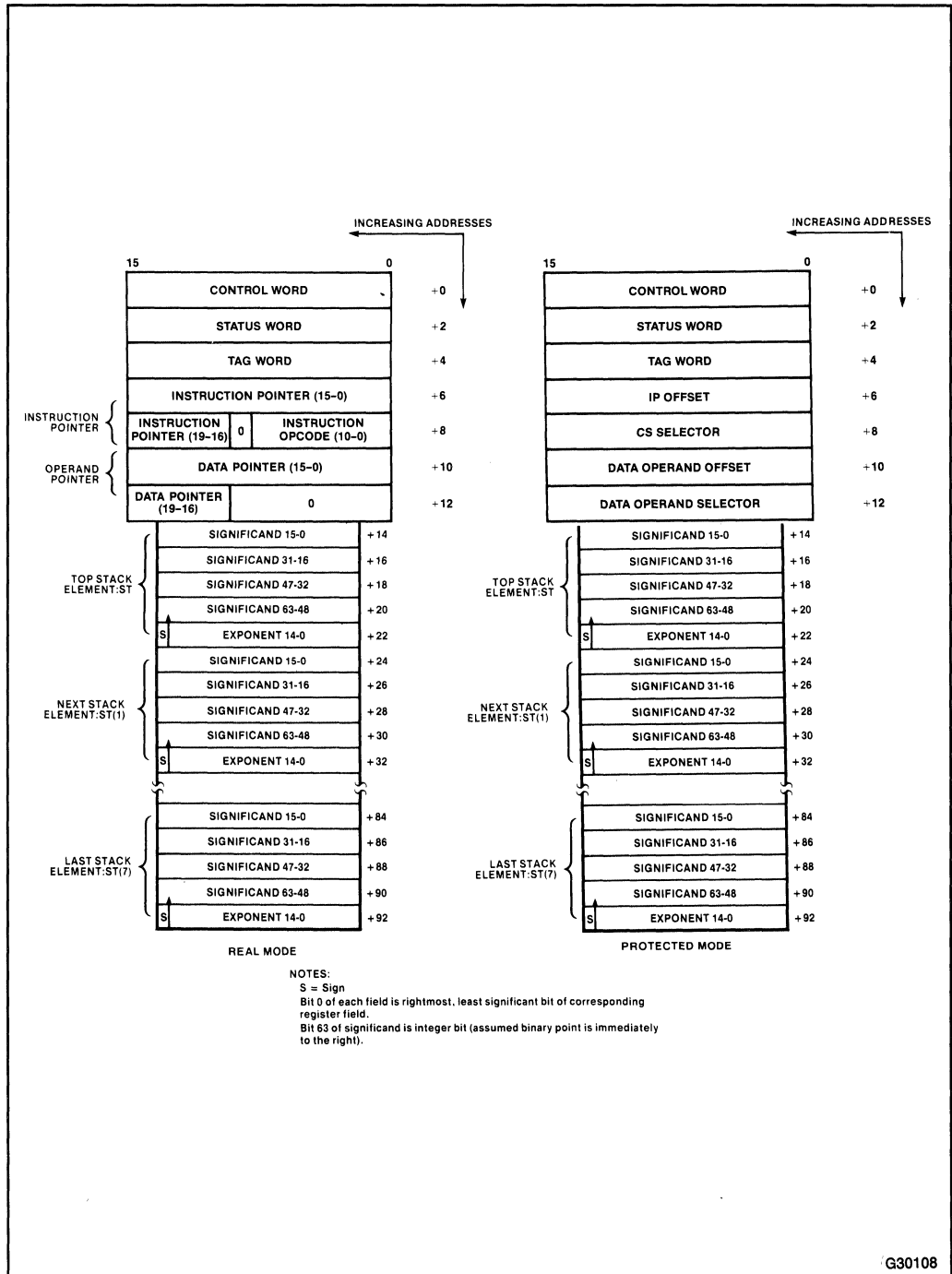
Figure 2-1. FSAVE/FRSTOR Memory Layout
