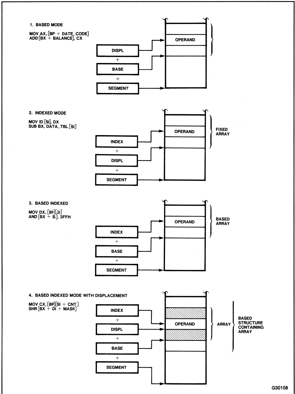
Figure 2-13. Complex Addressing Modes
