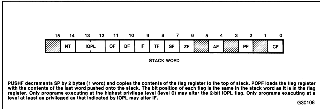
Figure 3-14. PUSHF and POPF
