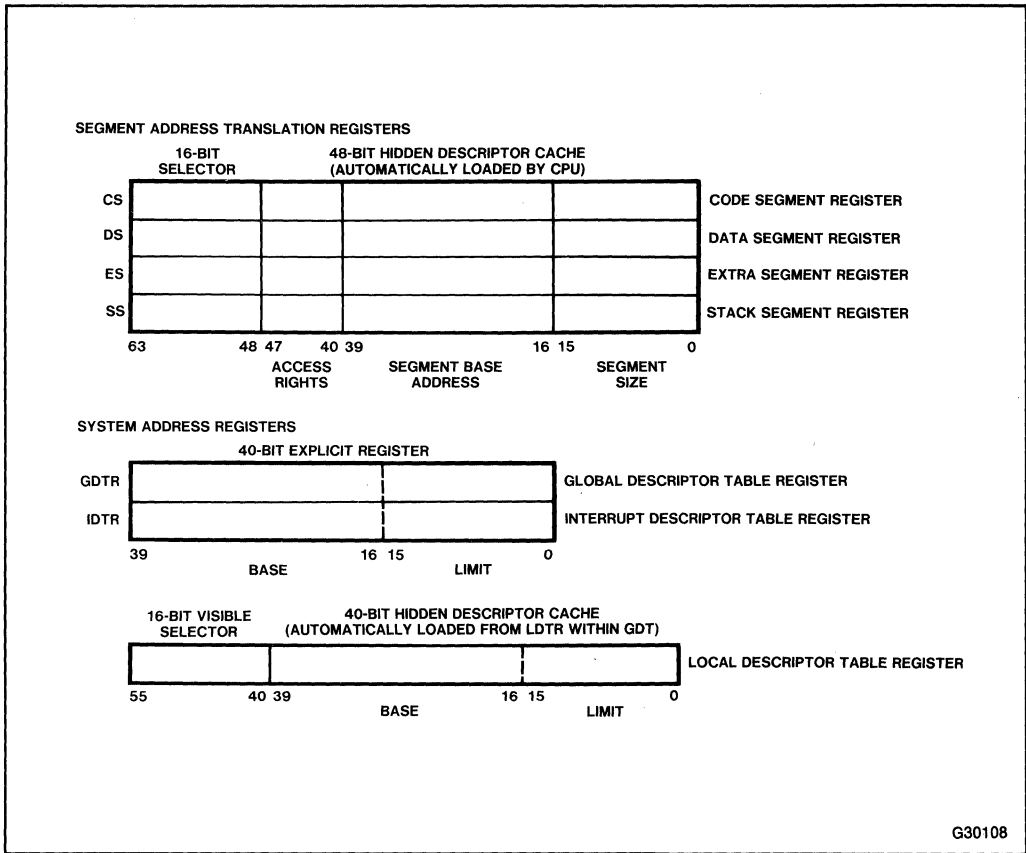
Figure 6-8. Memory Management Registers
