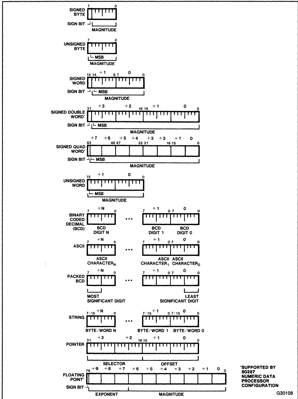
Figure 2-3. 80286/80287 Supported Data Types
