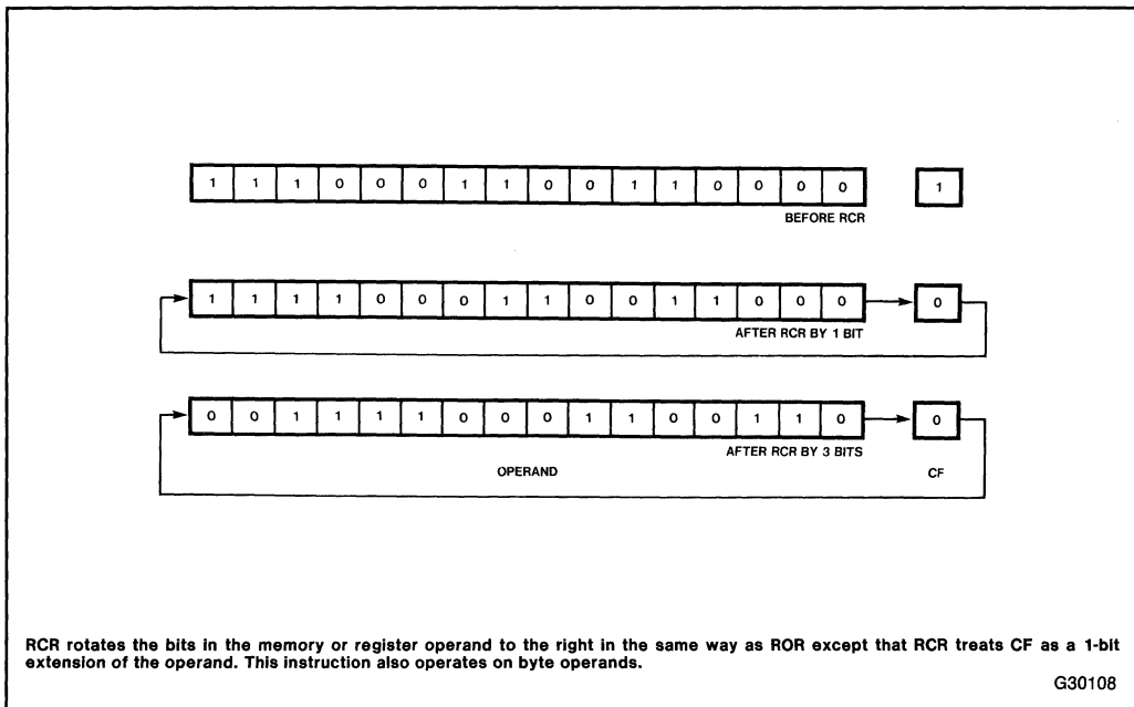
Figure 3-12. RCR
