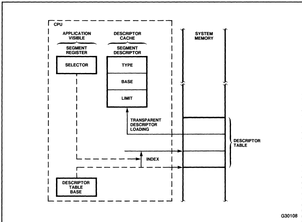
Figure 6-9. Descriptor Loading
