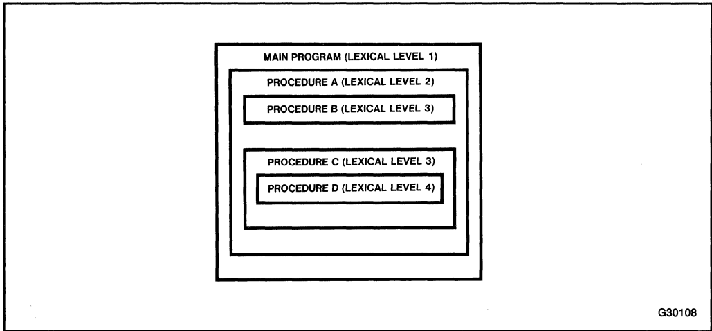
Figure 4-2. Variable Access in Nested Procedures
