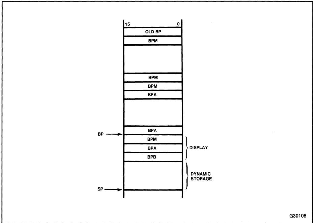
Figure 4-2d. Stack Frame for Procedure C at Level 3 Called from B
