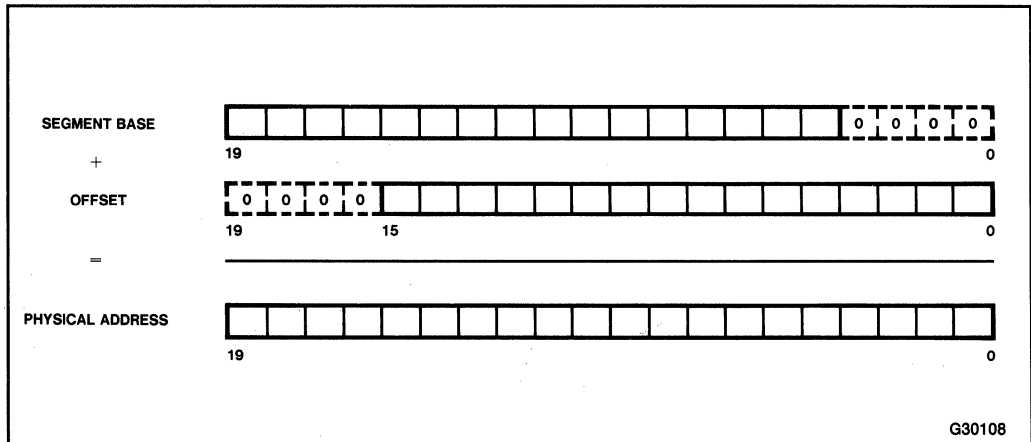
Figure 5-1b. Forming the 20-bit Physical Address in the Real Address Mode
