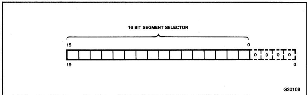
Figure 5-1a. Forming the Segment Base Address
