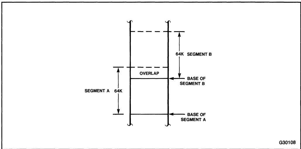
Figure 5-2. Overlapping Segments to Save Physical Memory
