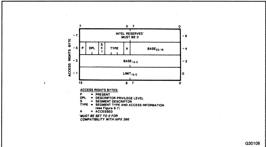
Figure 6-3. Code or Data Segment Descriptor (S = 1)
