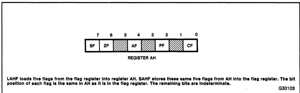
Figure 3-13. LAHF and SAHF
