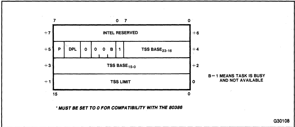
Figure 8-2. TSS Descriptor
