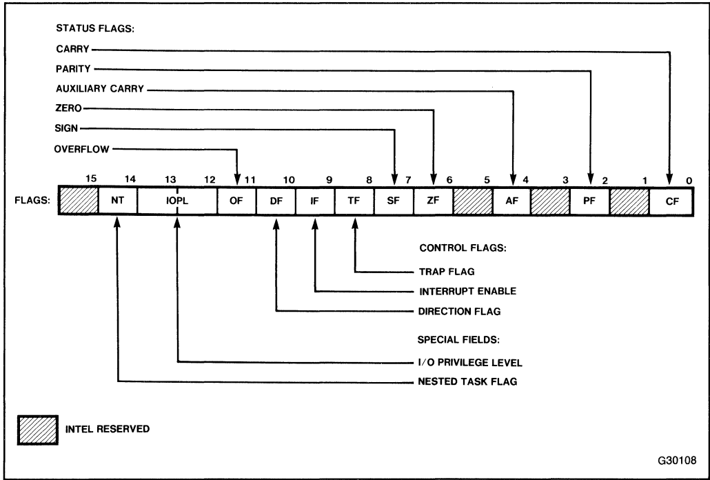
Figure 2-10. Flags Register
