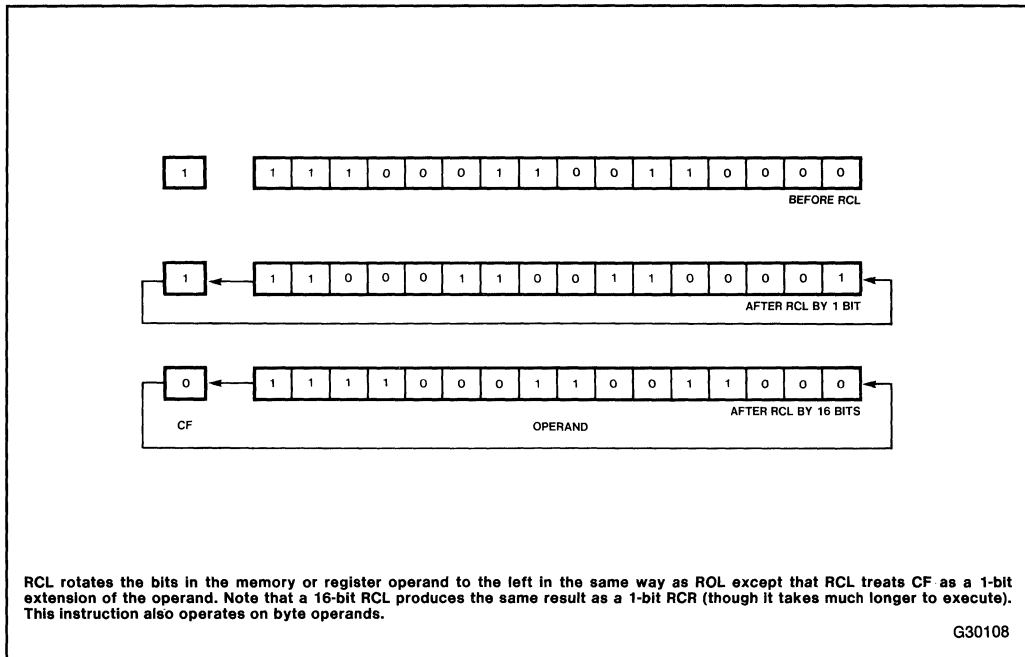
Figure 3-11. RCL
