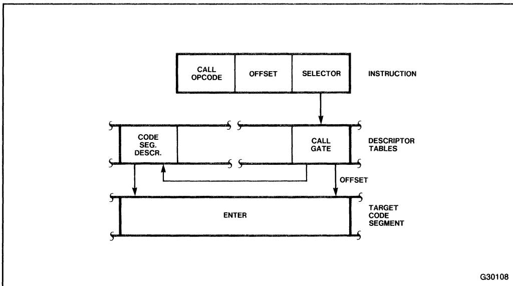
Figure 7-11. Call Gate
