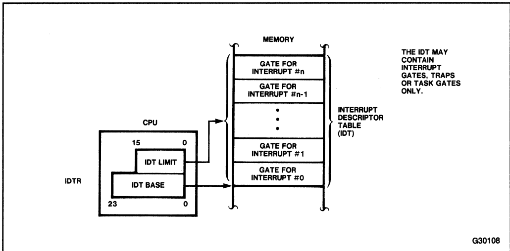
Figure 9-1. Interrupt Descriptor Table Definition
