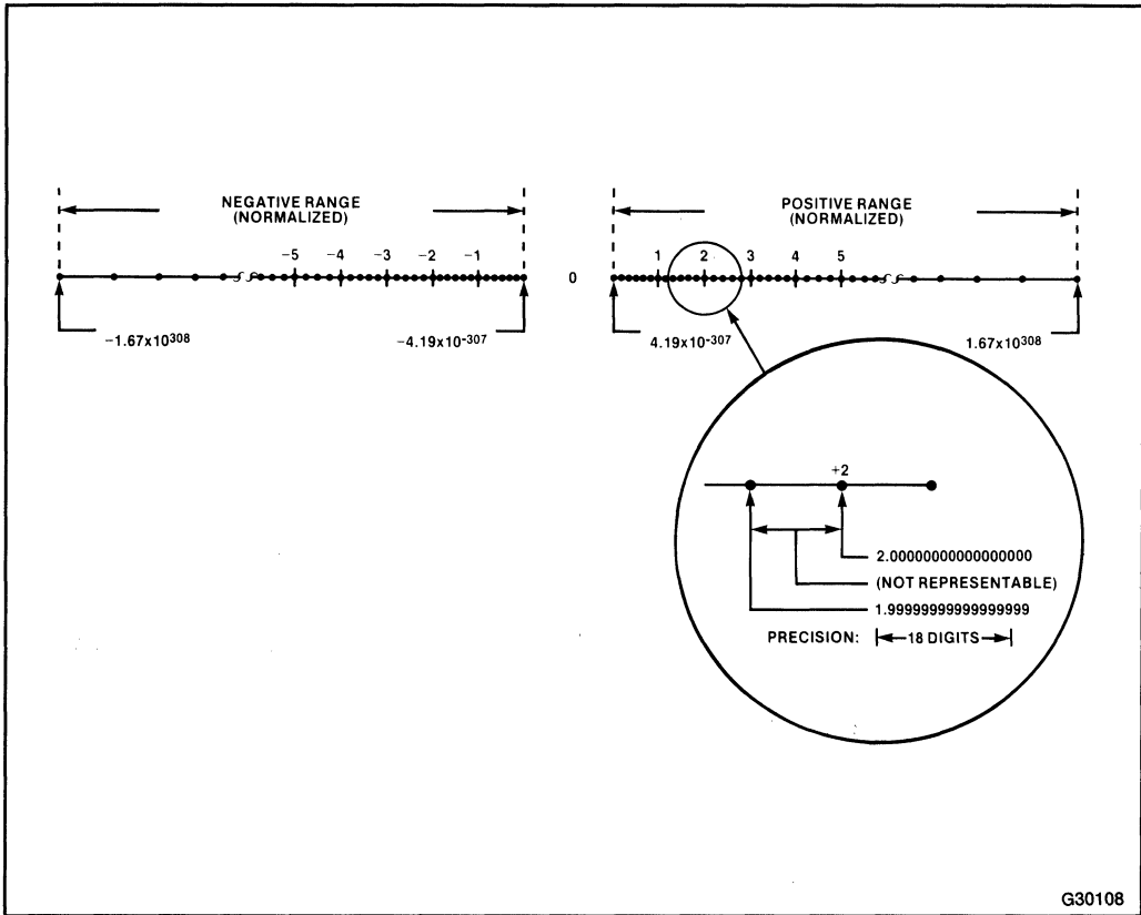
Figure 1-8. 80287 Number System
