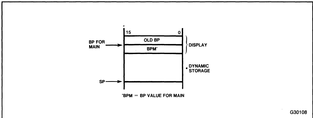
Figure 4-2a. Stack Frame for MAIN at Level 1
