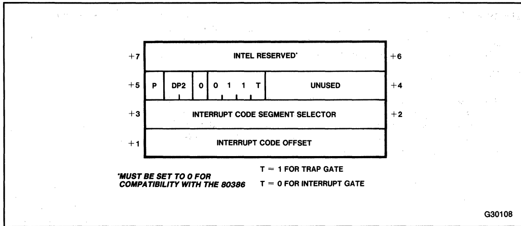
Figure 9-3. Trap/Interrupt Gate Descriptors
