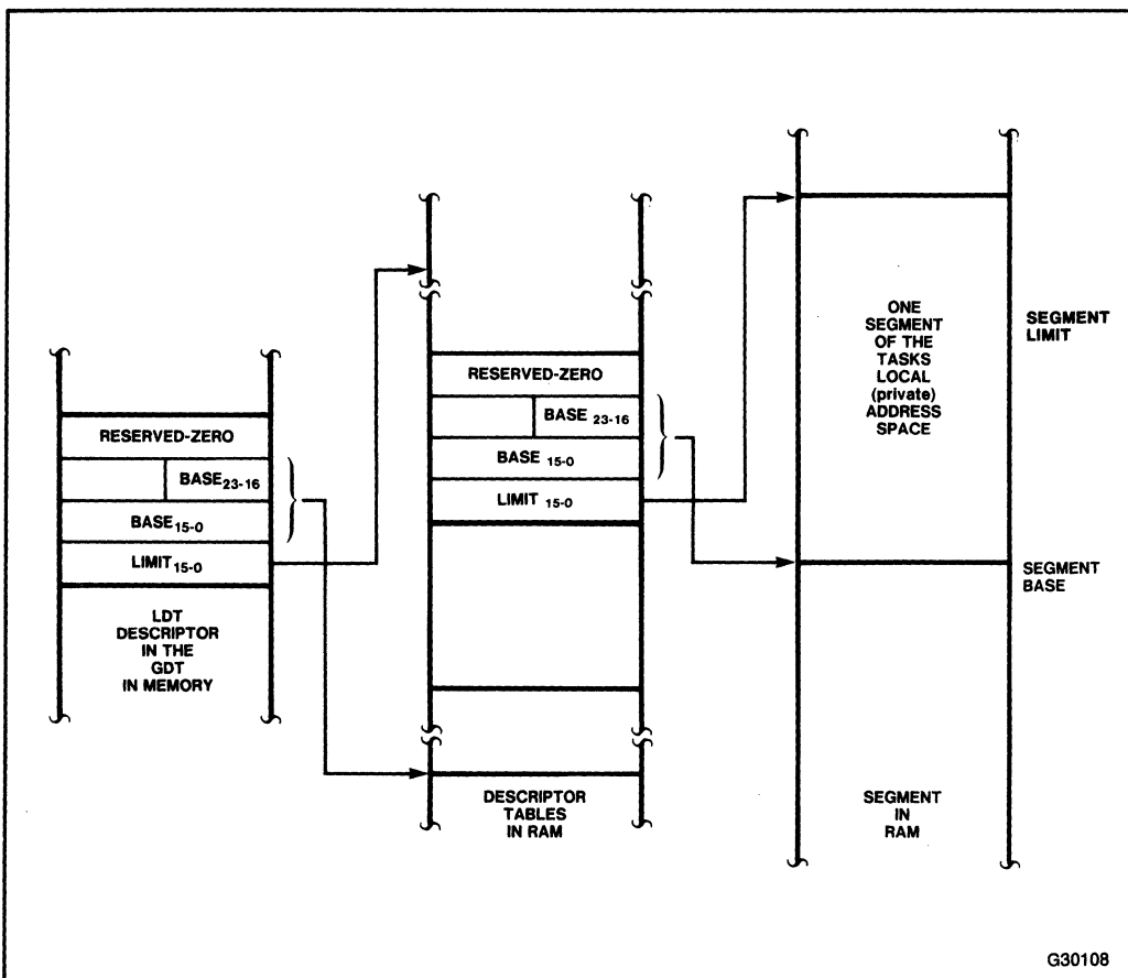
Figure 6-5. LDT Descriptor
