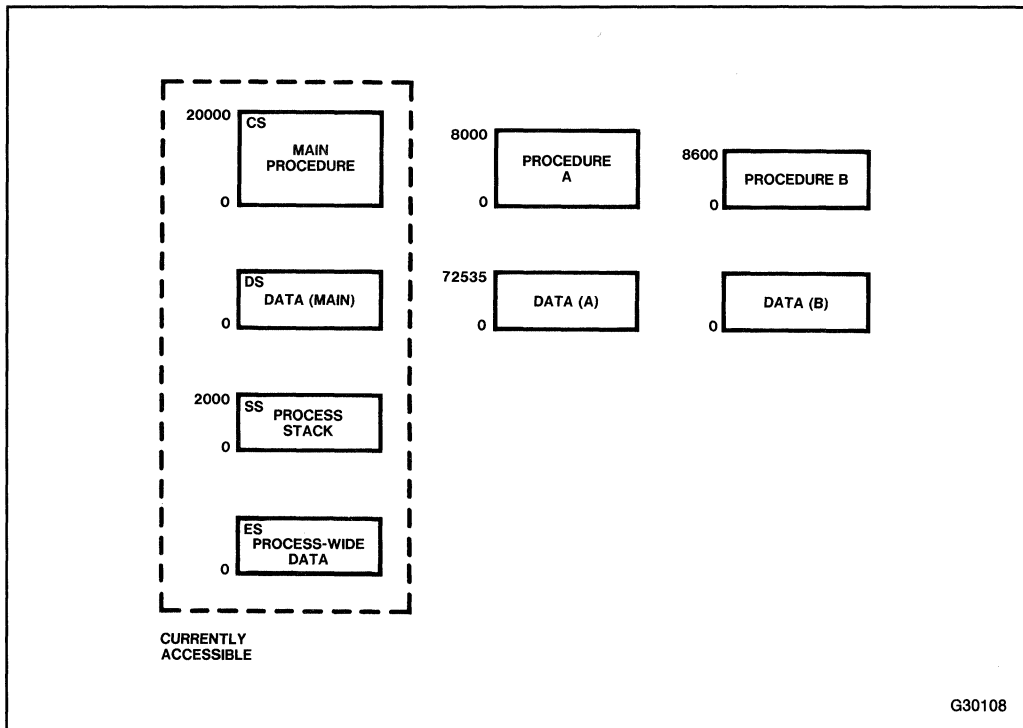
Figure 2-1. Segmented Virtual Memory
