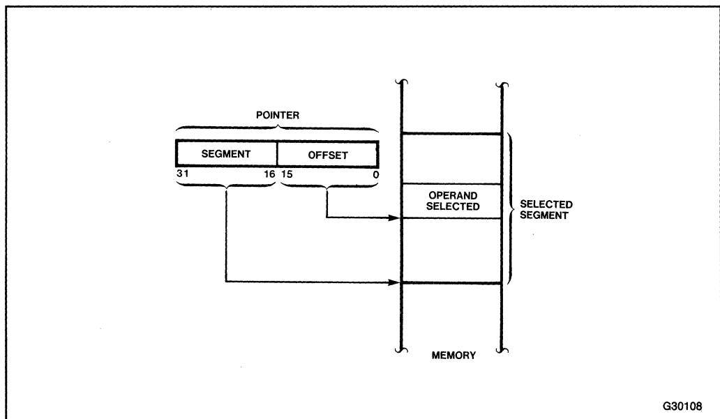
Figure 2-11. Two-Component Address
