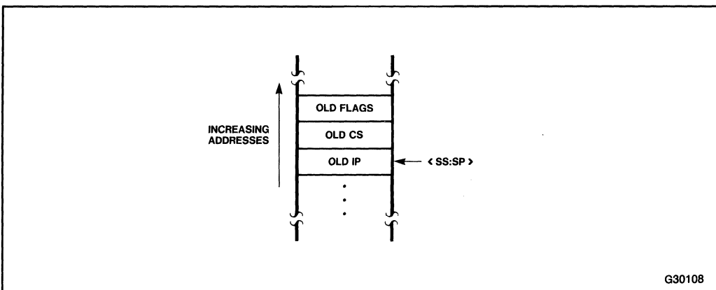
Figure 5-4. Stack Structure after Interrupt (Real Address Mode)
