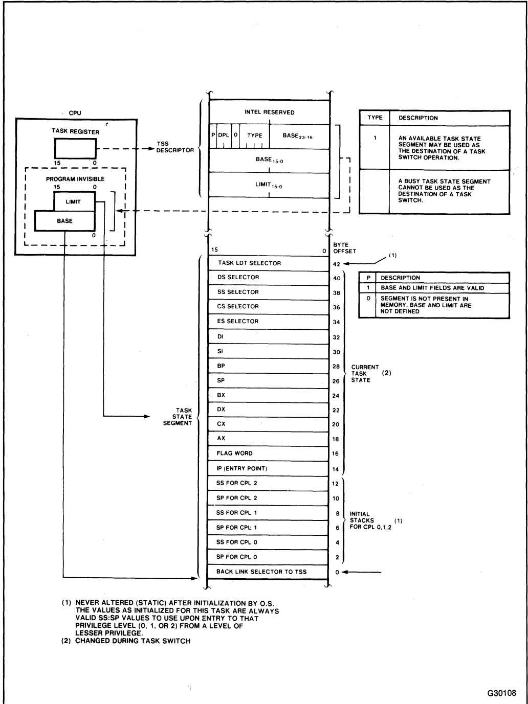
Figure 8-1. Task State Segment and TSS Registers
