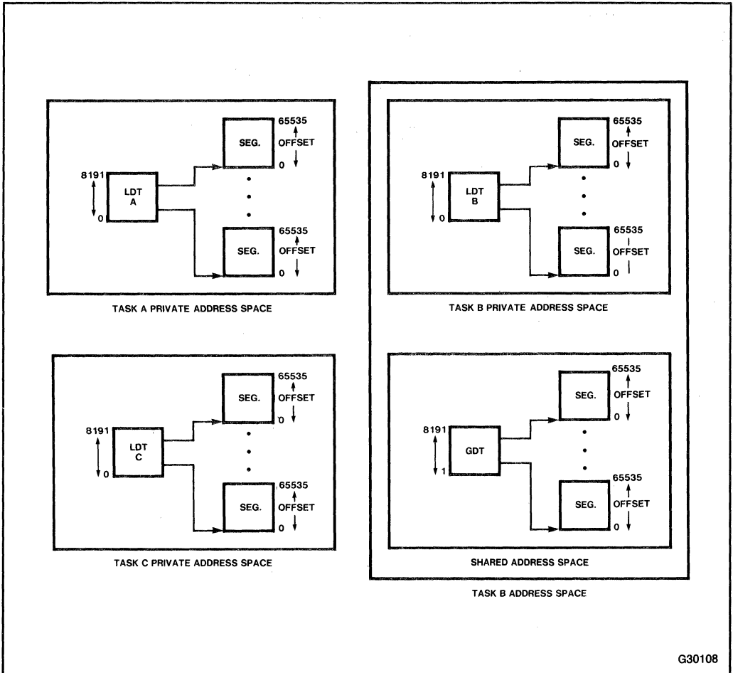
Figure 7-3. 80286 Virtual Address Space
