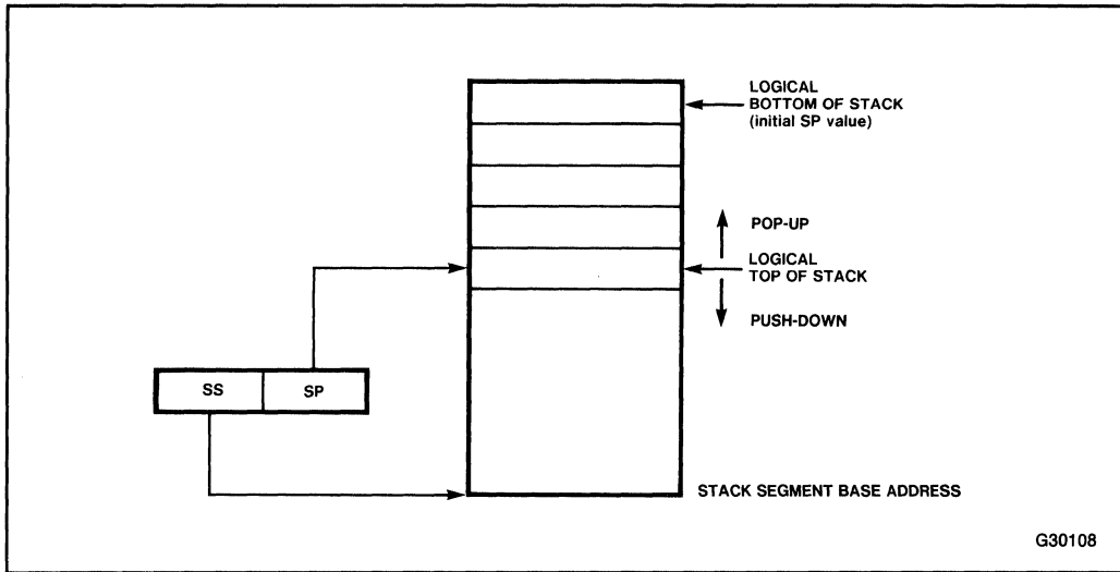
Figure 2-7. 80286 Stack
