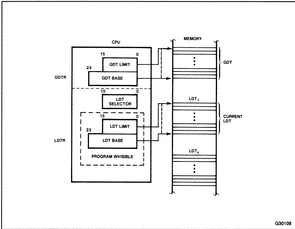
Figure 7-4. Local and Global Descriptor Table Definitions
