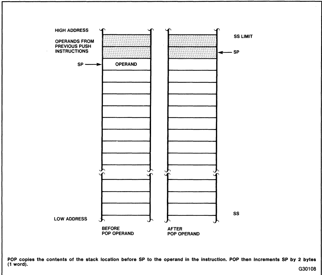
Figure 3-3. POP
