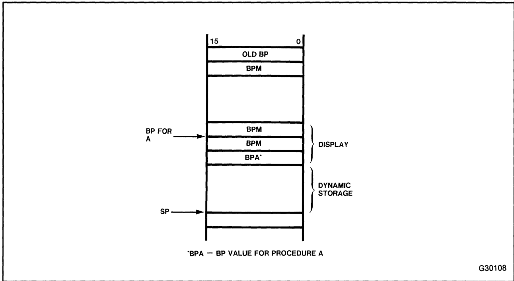
Figure 4-2b. Stack Frame for Procedure A
