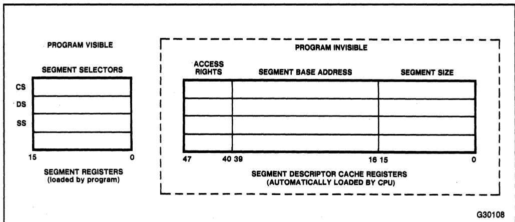
Figure 7-2. Descriptor Cache Registers
