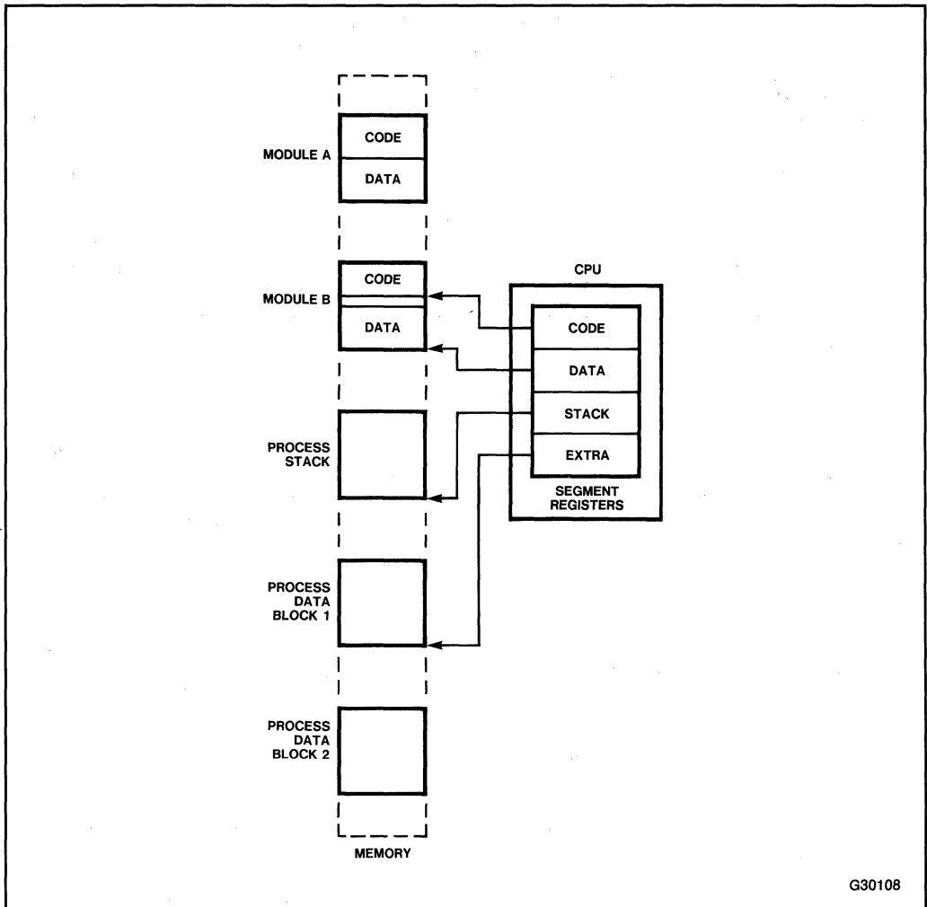
Figure 2-12. Use of Memory Segmentation
