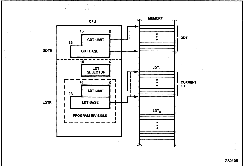
Figure 10-1. Local and Global Descriptor Table Definition
