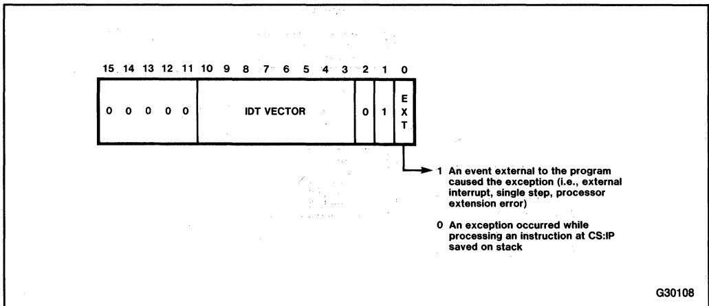
Figure 9-2. IDT Selector Error Code
