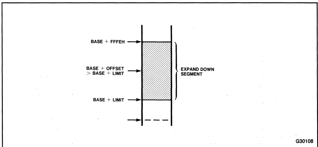
Figure 11-1. Expand-Down Segment
