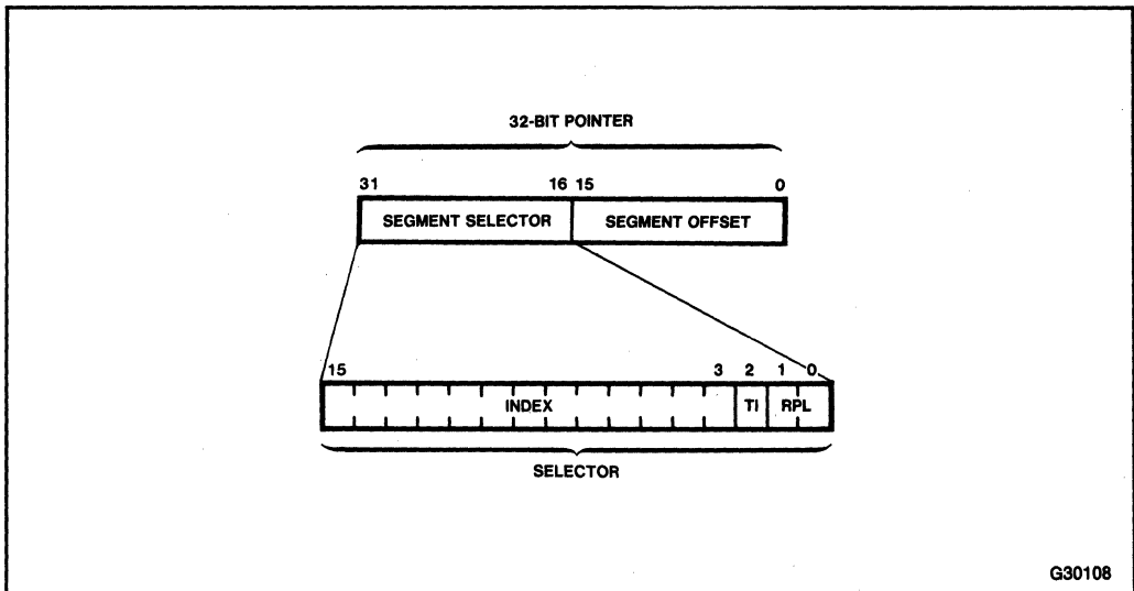
Figure 6-1. Format of the Segment Selector Component
