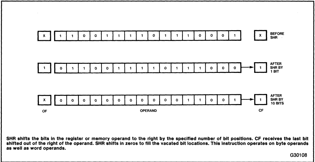
Figure 3-7. SHR
