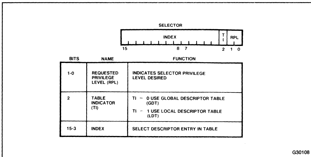
Figure 7-7. Selector Fields
