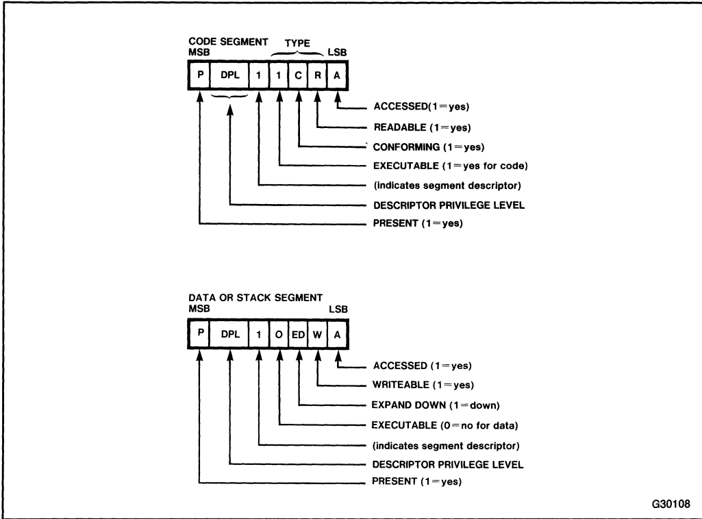
Figure 6-7. Segment Descriptor Access Bytes
