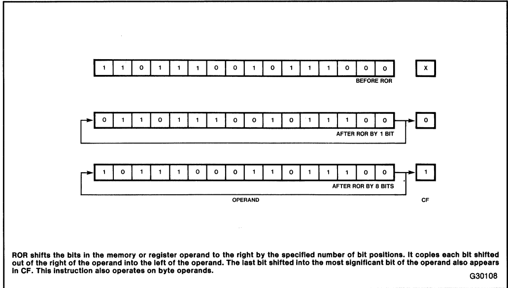
Figure 3-10. ROR
