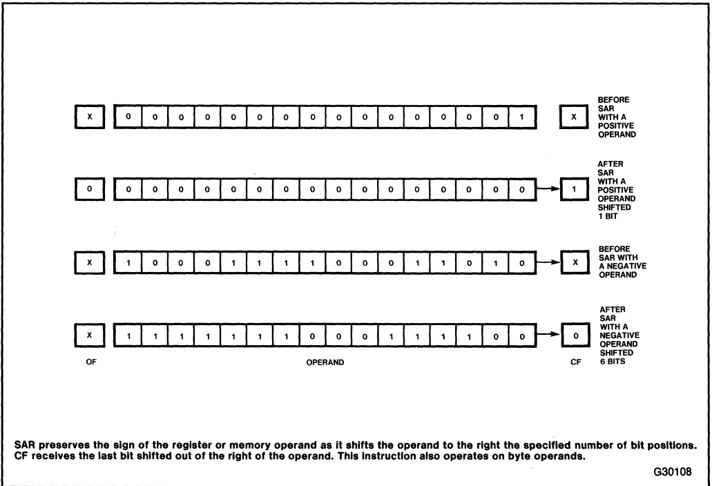
Figure 3-8. SAR
