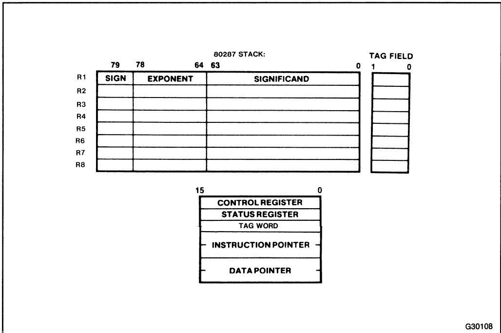
Figure 1-3. 80287 Register Set
