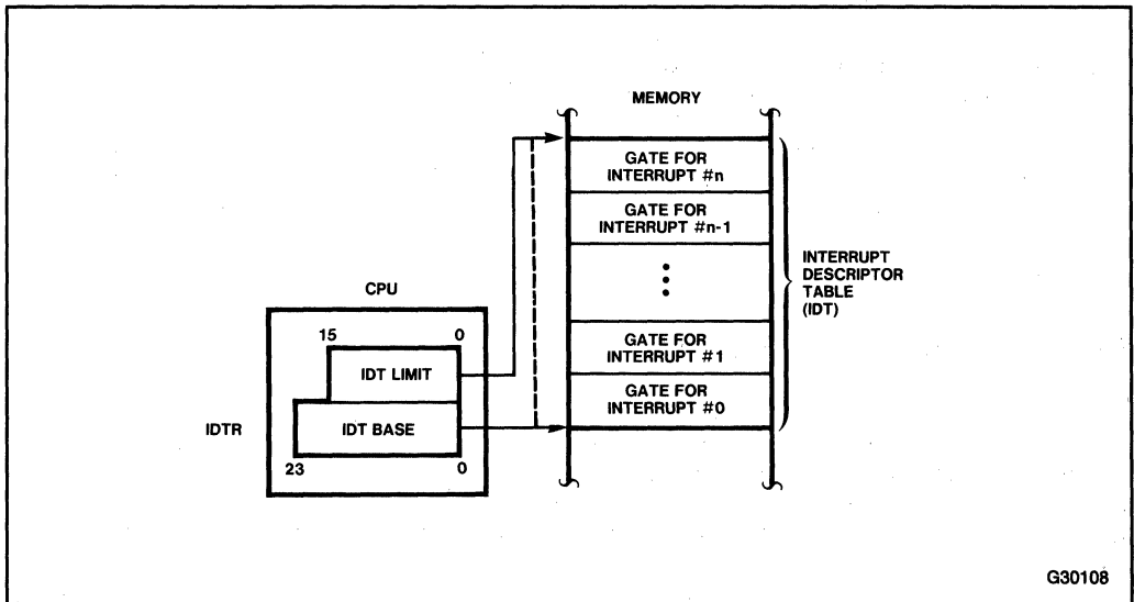
Figure 10-2. Interrupt Descriptor Table Definition
